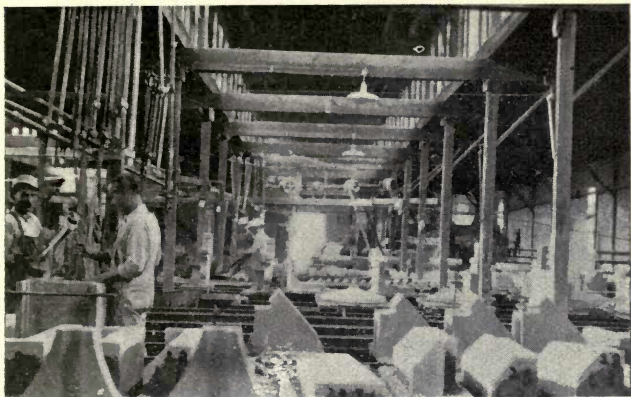
FIG. 37—VIEW OF MOLDING ROOM OF TRIM STONE FACTORY—NOTE MOLD BEING FILLED AND CONCRETE TAMPED AT LEFT
